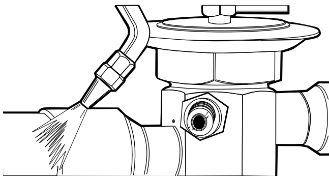
Fig. 107 — Solder Technique
