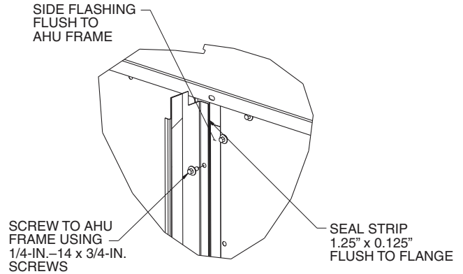
Fig. 64 — Screw the Side Flashings to Unit
