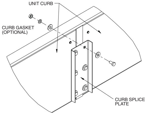
Fig. 20 — Splice Plate Usage
