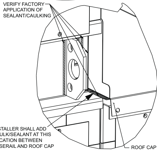
Fig. 159 — Verify Seals (6 in. baserail shown)
