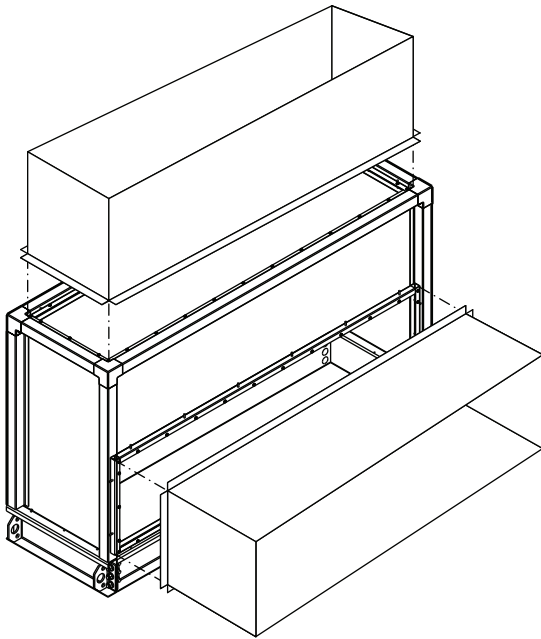
Fig. 38 — Duct Connections — Mixing Box Ductwork Attachment
