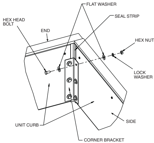
Fig. 21 — Corner Bracket
