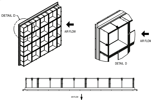
Fig. 205 — HEPA Holding Frame, Sizes 72 to 110
