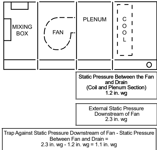
Fig. 116 — Blow-Thru Example
