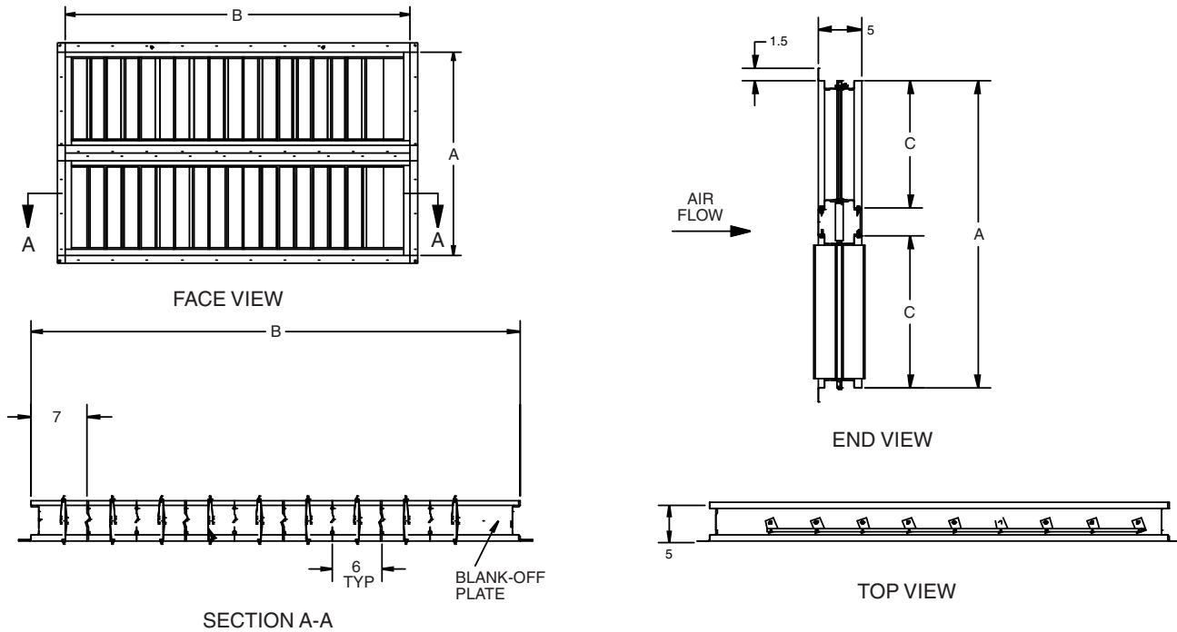
Fig. 46 — 39M06-61 Unit Zone Damper Section Details
