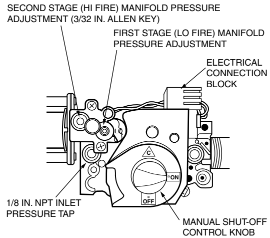
Fig. 151 — 2-Stage Gas Valve
