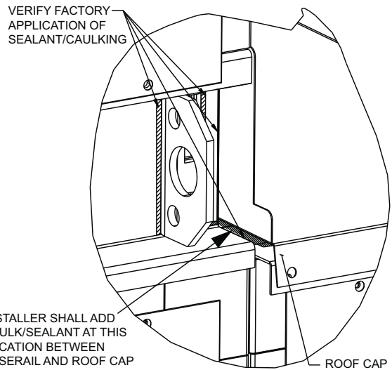
Fig. 169 — Apply Sealant/Caulk to Joints
