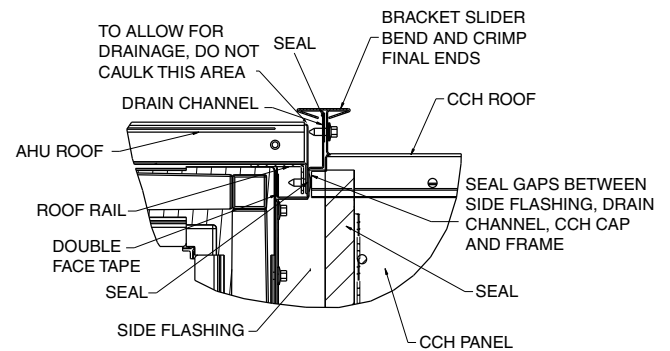
Fig. 68 — Screwing CCH Roof to Drain Channel
