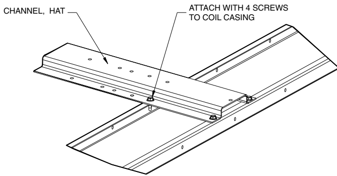
Fig. 95 — Secure Spacer
