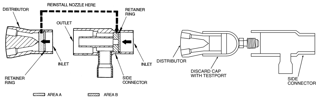
Fig. 109 — Distributor and Hot Gas Bypass Auxiliary Side Connector
