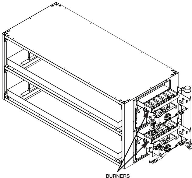
Fig. 141 — Gas-Fired Rack System Burner Assembly
