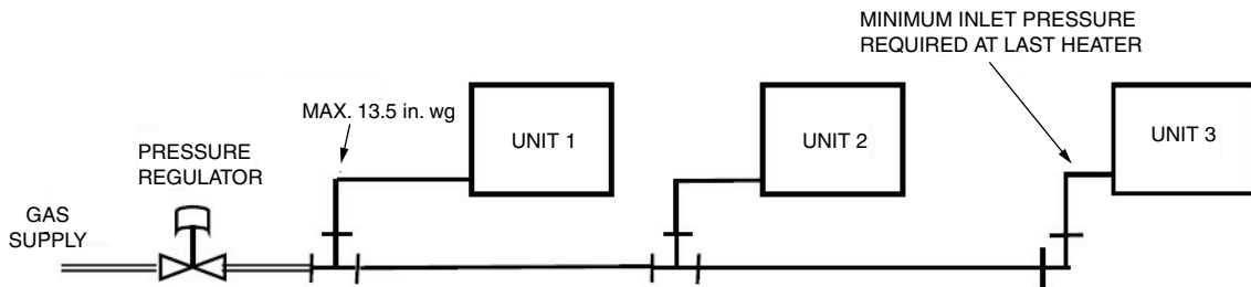
Fig. 148 — Inlet Pressure for Multiple Heaters
