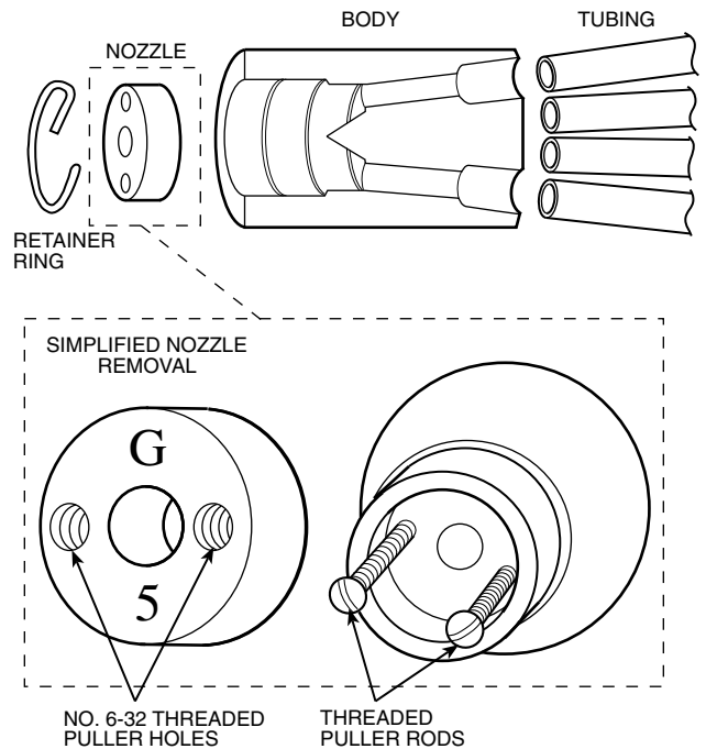
Fig. 106 — Nozzle Change-Out
