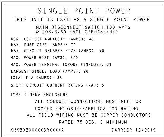
Fig. 174 — Connection of Power to Single Point Power Enclosure
