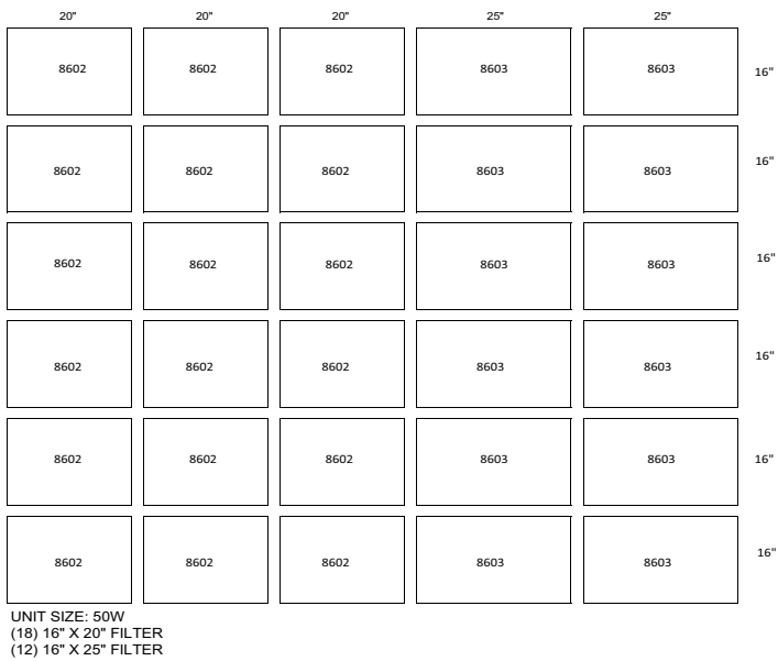
Fig. 207 — Filter Mixing Box and Angle Filter Arrangement — 2-in. or 4-in. (cont)
