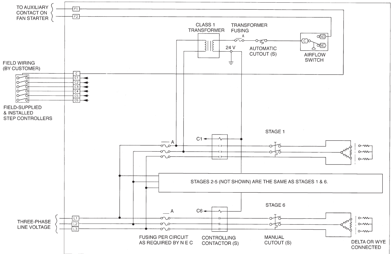
Fig. 137 — Electrical Heater Wiring Schematic (Typical)
