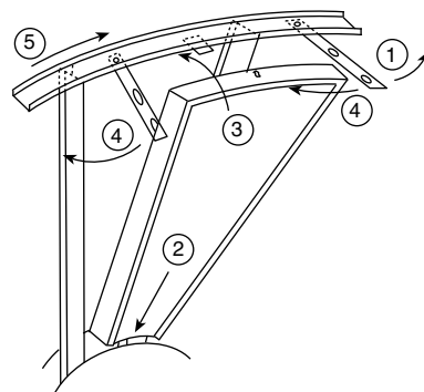
Fig. 187 — Segment Installation
