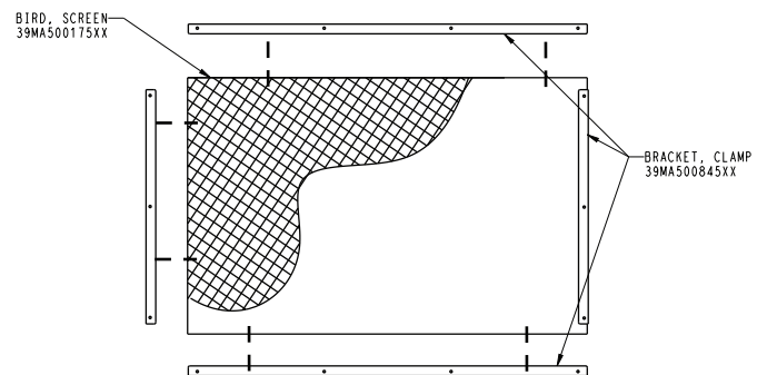
Fig. 80 — Mounting the Bird Screen
