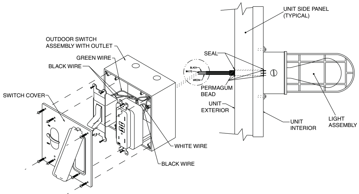
Fig. 171 — Marine Light with Convenience Outlet and Switch, Outdoor Installation
