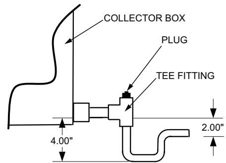
Fig. 143 — Condensate Drain
