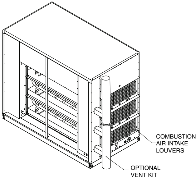
Fig. 156 — Indoor Venting with Flue Riser Kit
