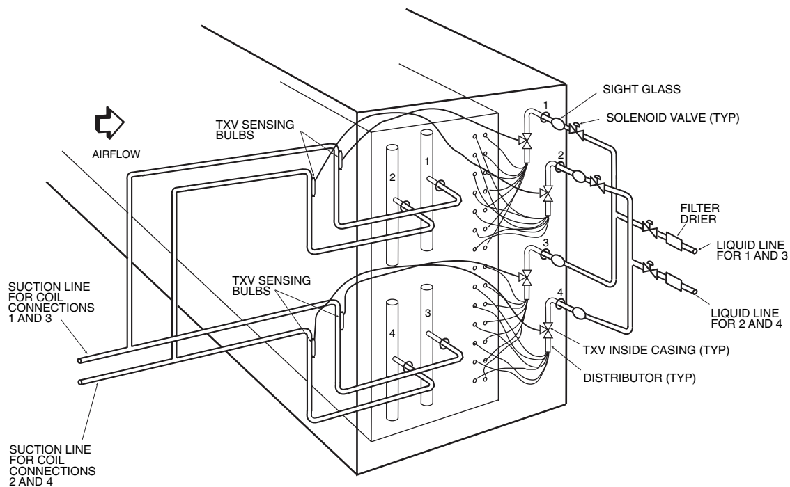
Fig. 111 — Row-Split Coil Manifolding (Typical)
