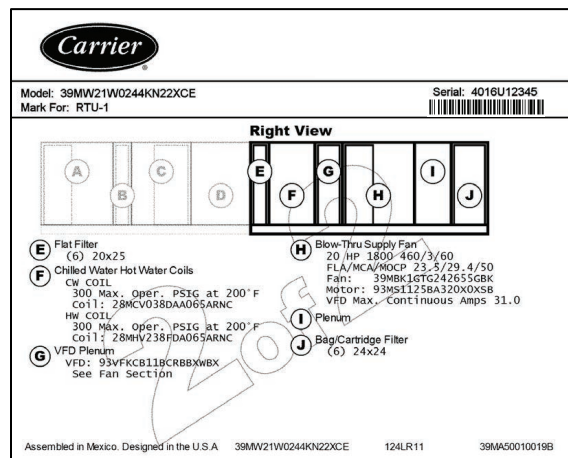
Fig. 2 — 39MW Unit Nameplate Label
