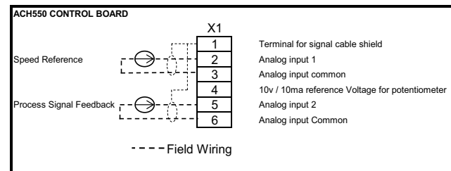
Fig. 133 — ACH550 Control Board Wiring
