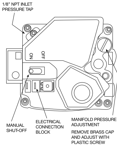
Fig. 150 — On/Off (1-Stage) Gas Valve
