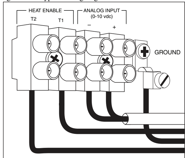
Fig. 142 — Gas-Fired Duct System Furnace Typical Wiring Diagram
