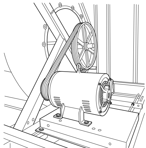
Fig. 211 — Fan Shaft and Bearing Removal
