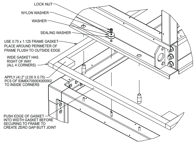
Fig. 161 — Verify Gasket Installation
