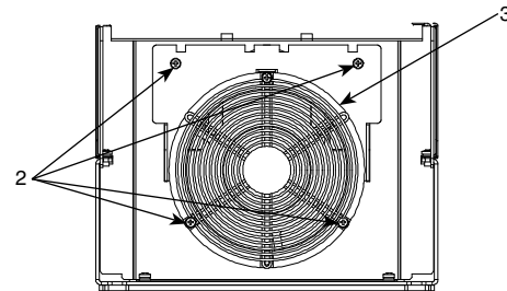
Fig. 213 — Main Fan Replacement (Frame Sizes R5 and R6)
