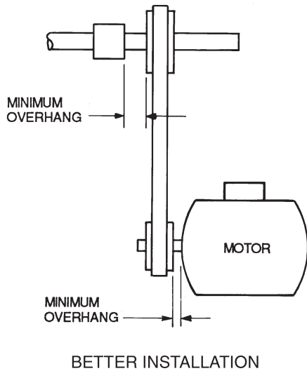
Fig. 54 — Determining Sheave-Shaft Overhang
