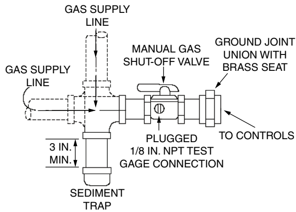
Fig. 149 — Sediment Trap, Shut-Off Valve, and Union
