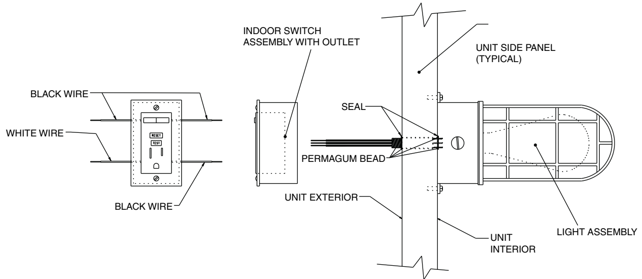
Fig. 170 — Marine Light with Convenience Outlet and Switch, Indoor Installation
