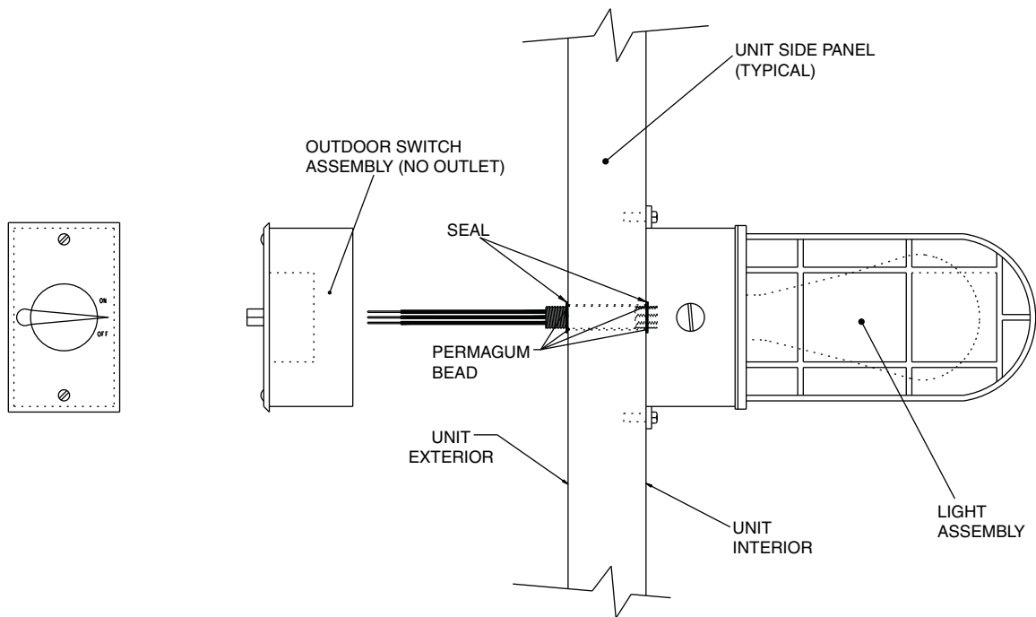
Fig. 173 — Marine Light with Switch (No Convenience Outlet), Outdoor Installation
