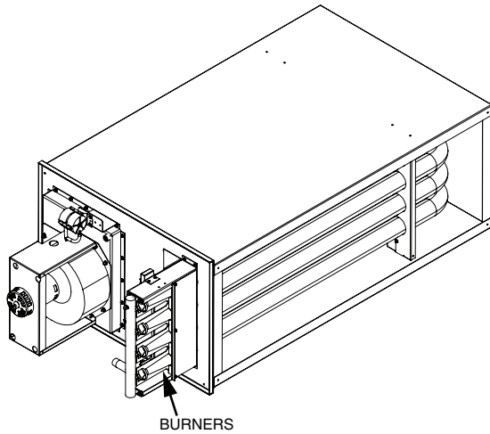
Fig. 140 — Gas-Fired Duct Furnace Burner Assembly
