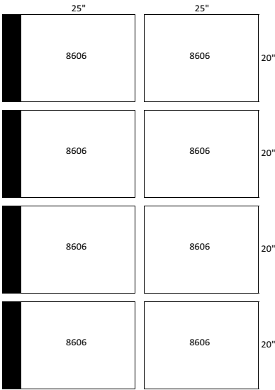
UNIT SIZE: 18T (8) 20" X 25" FILTERS
