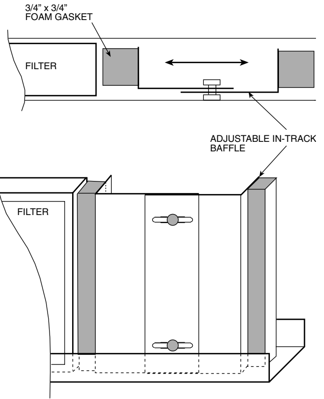
Fig. 203 — In-Track Baffle for Flat, Angle and Sideloading Bag/Cartridge Filter Sections
