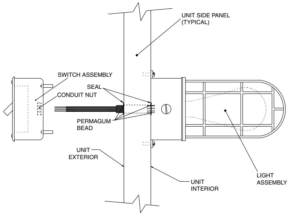
Fig. 172 — Marine Light with Switch (No Convenience Outlet), Indoor Installation
