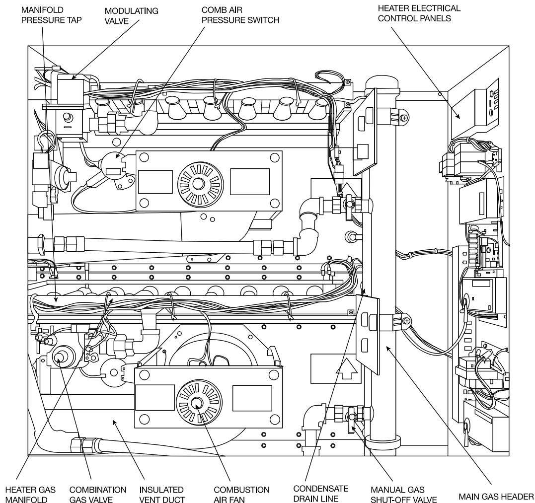
Fig. 154 — Gas-Fired Rack Furnace Components
