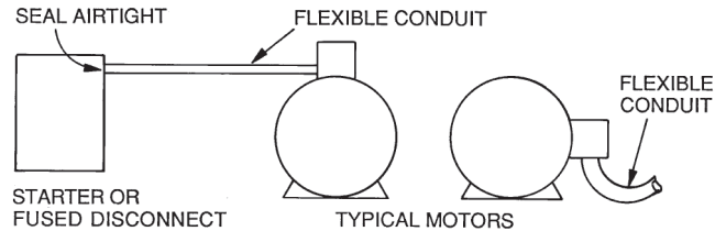
Fig. 53 — Sealing Power Wires in Flexible Conduit
