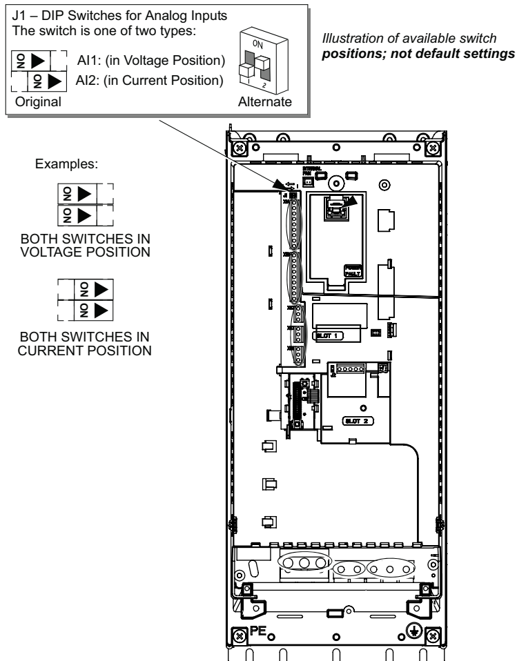
Fig. 121 — Setting AI Switch to Voltage Position
