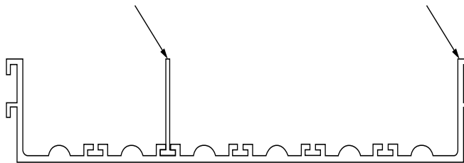
Fig. 202 — 6-in. Track Assembly
