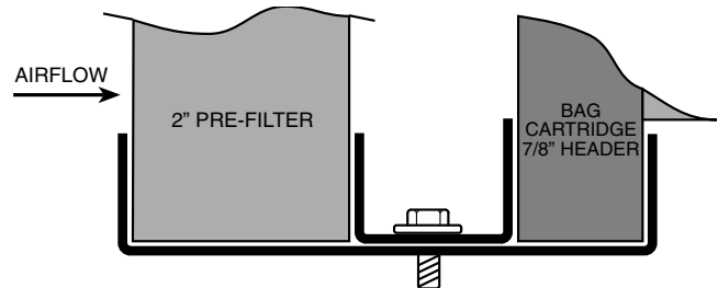
Fig. 200 — Track for Draw-Thru Bag Cartridge Filter Section
