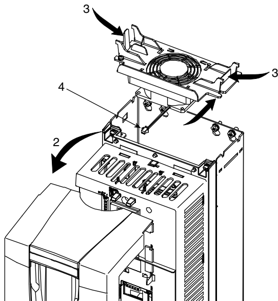
Fig. 212 — Main Fan Replacement (Frame Sizes R1 - R4)
