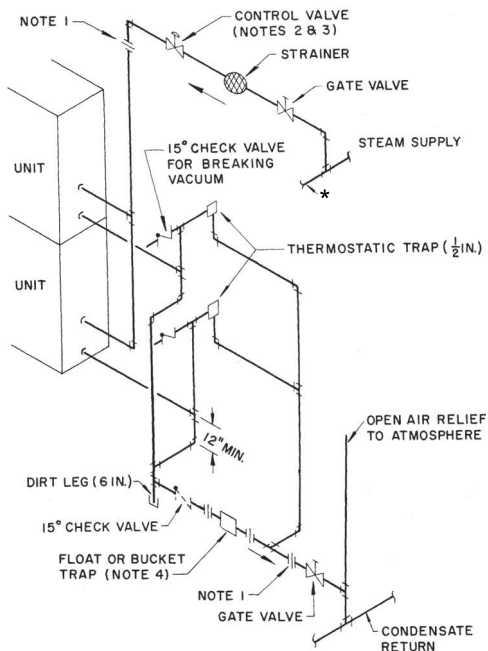
Fig. 100 — Multiple Coil High Pressure Piping
