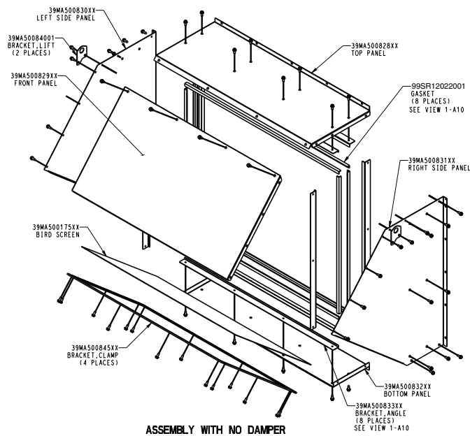
Fig. 72 — Exploded Power Exhaust Hood Assembly without Damper (Size 36 Shown)
