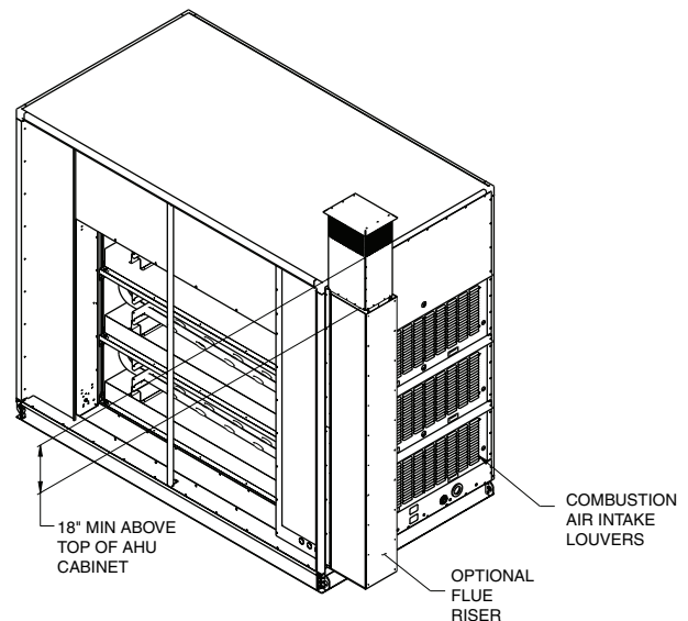
Fig. 155 — Outdoor Venting with Flue Riser Kit
