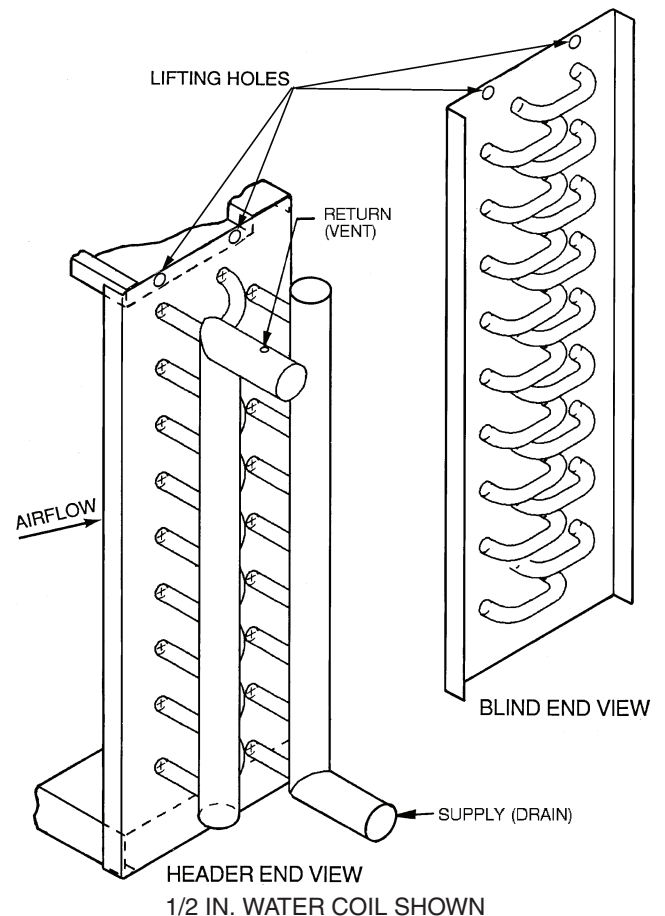
Fig. 97 — Coil Connections and Lifting Points
