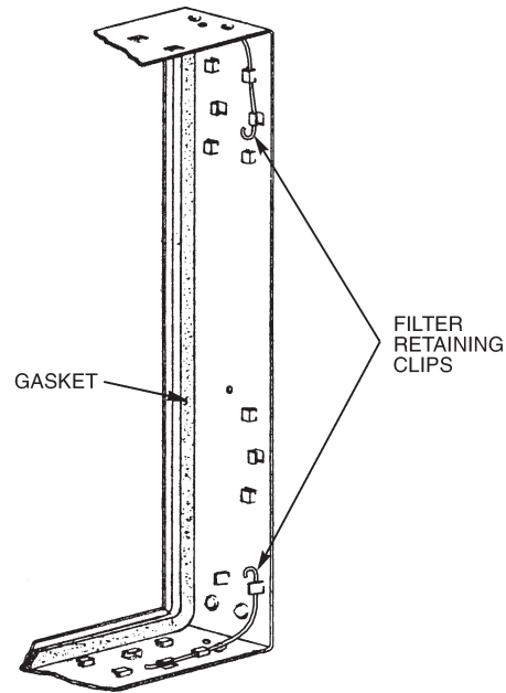
Fig. 199 — Puro-Frame Holding Frame and Filter Retaining Clips
