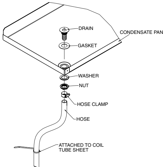
Fig. 96 — Install Drain Fittings
