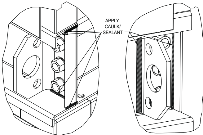
Fig. 160 — ERV Arrangement Sealant
