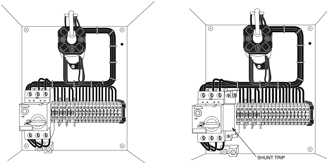
Fig. 130 — MMS Before and After Shunt Trip Installation
