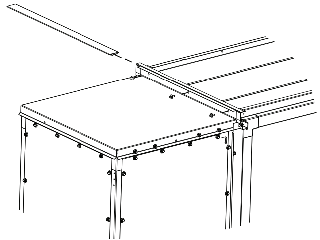
Fig. 68 — Screwing CCH Roof to Drain Channel
