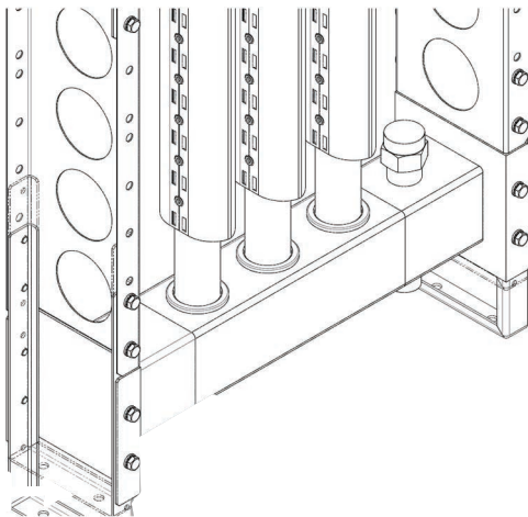
Fig. 92 — Vertical Manifold
