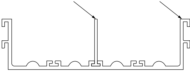
Fig. 201 — 2-in. Track Assembly (4-in. Track)
