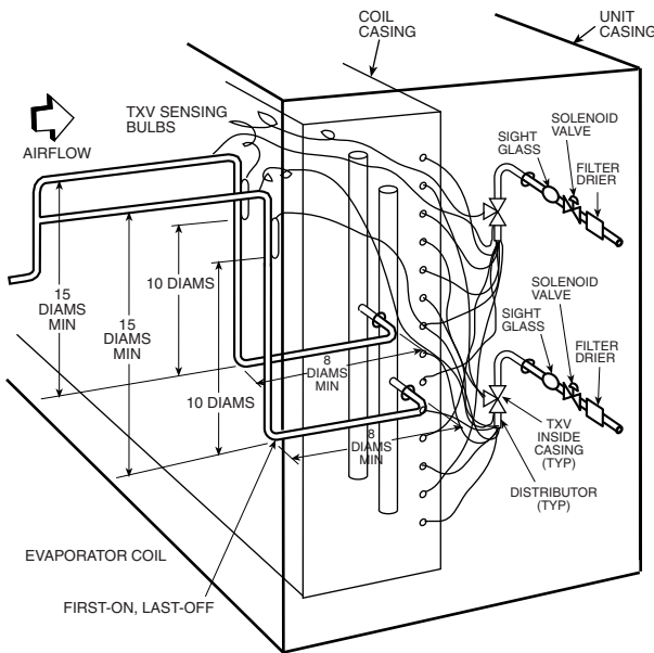
Fig. 103 — Face Split Coil Suction-Line Piping
