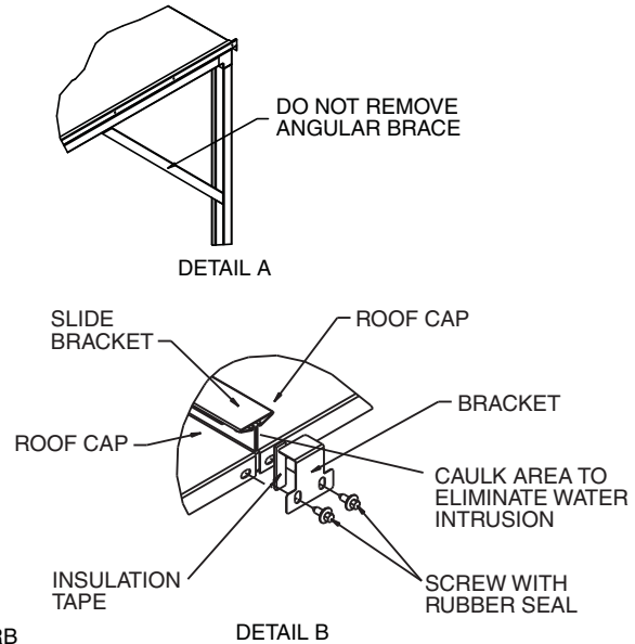
Fig. 32 — 39MW Split Assembly
