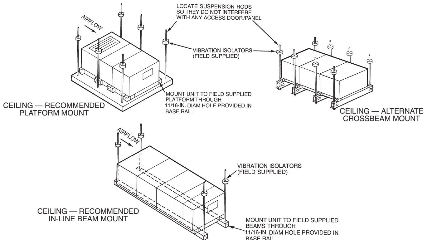
Fig. 16 — Unit Suspension
