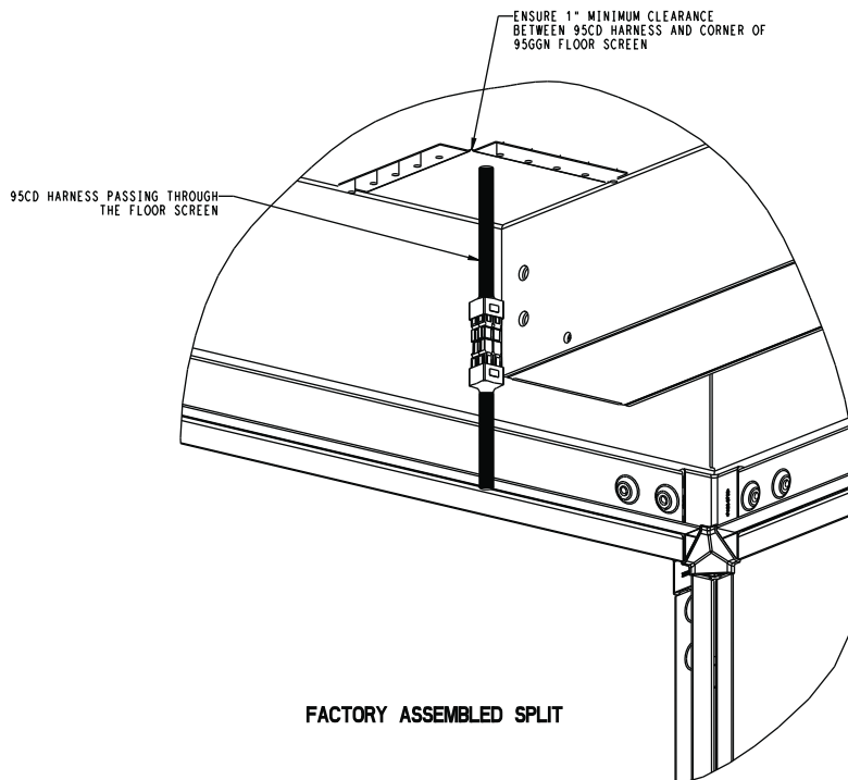
Fig. 35 — Stacked Unit Harness Connection at Vertical Split as Assembled
