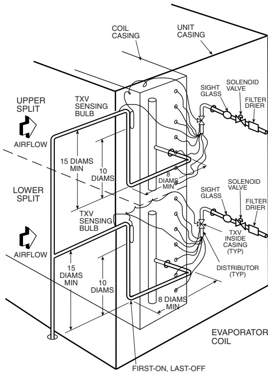
Fig. 103 — Face Split Coil Suction-Line Piping
