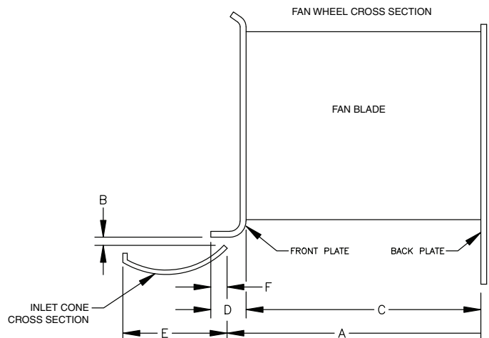
Fig. 15 — Plenum Fan Wheel and Inlet Cone Dimensions
