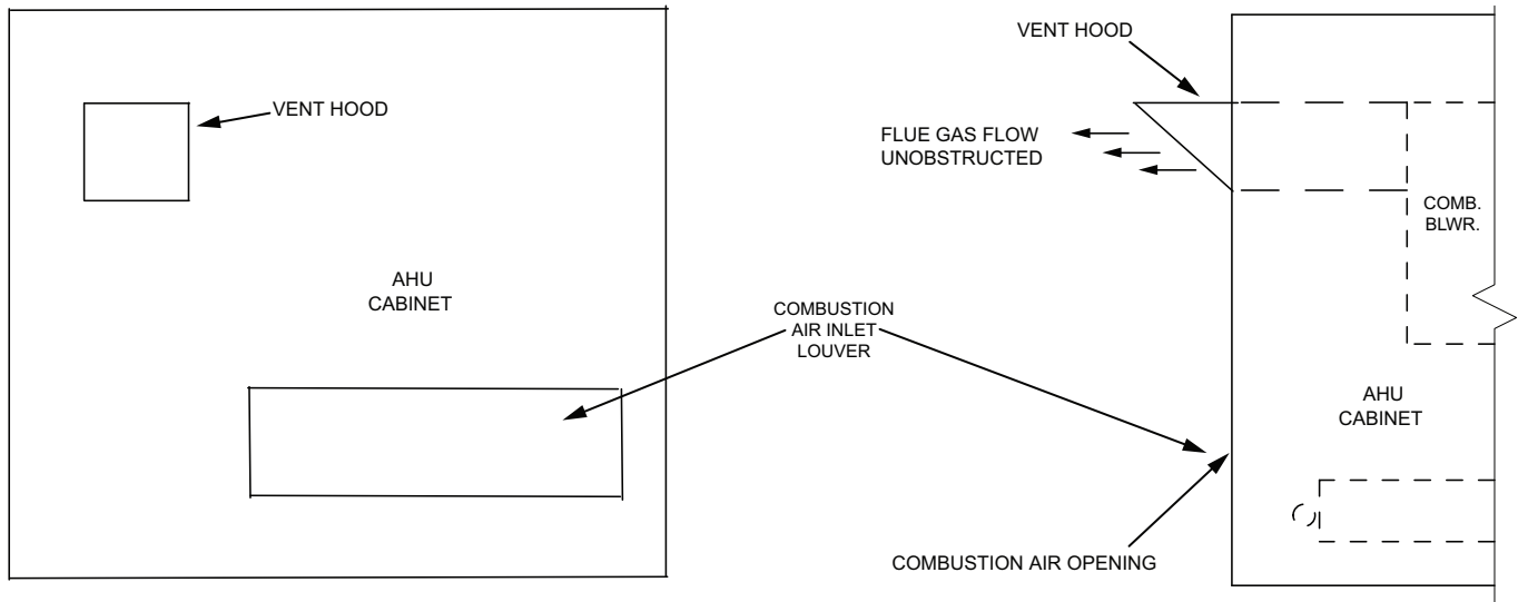
Fig. 145 — Outdoor Horizontal Venting
