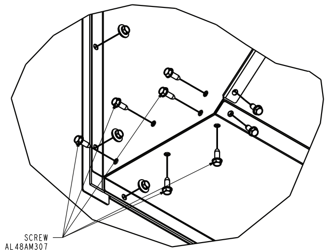
Fig. 79 — Securing the Bottom Panel
