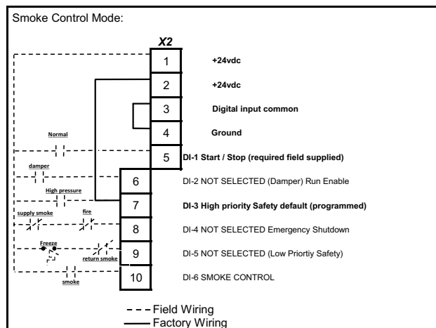
Fig. 136 — Smoke Detector Typical Wiring Diagram
