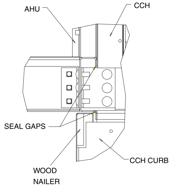
Fig. 69 — Side View
