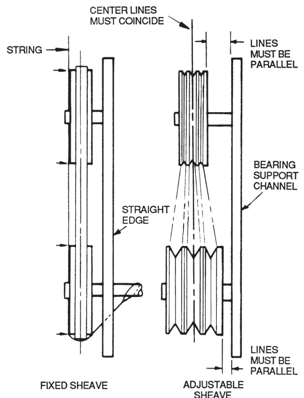
Fig. 55 — Determining Sheave-Shaft Alignment
