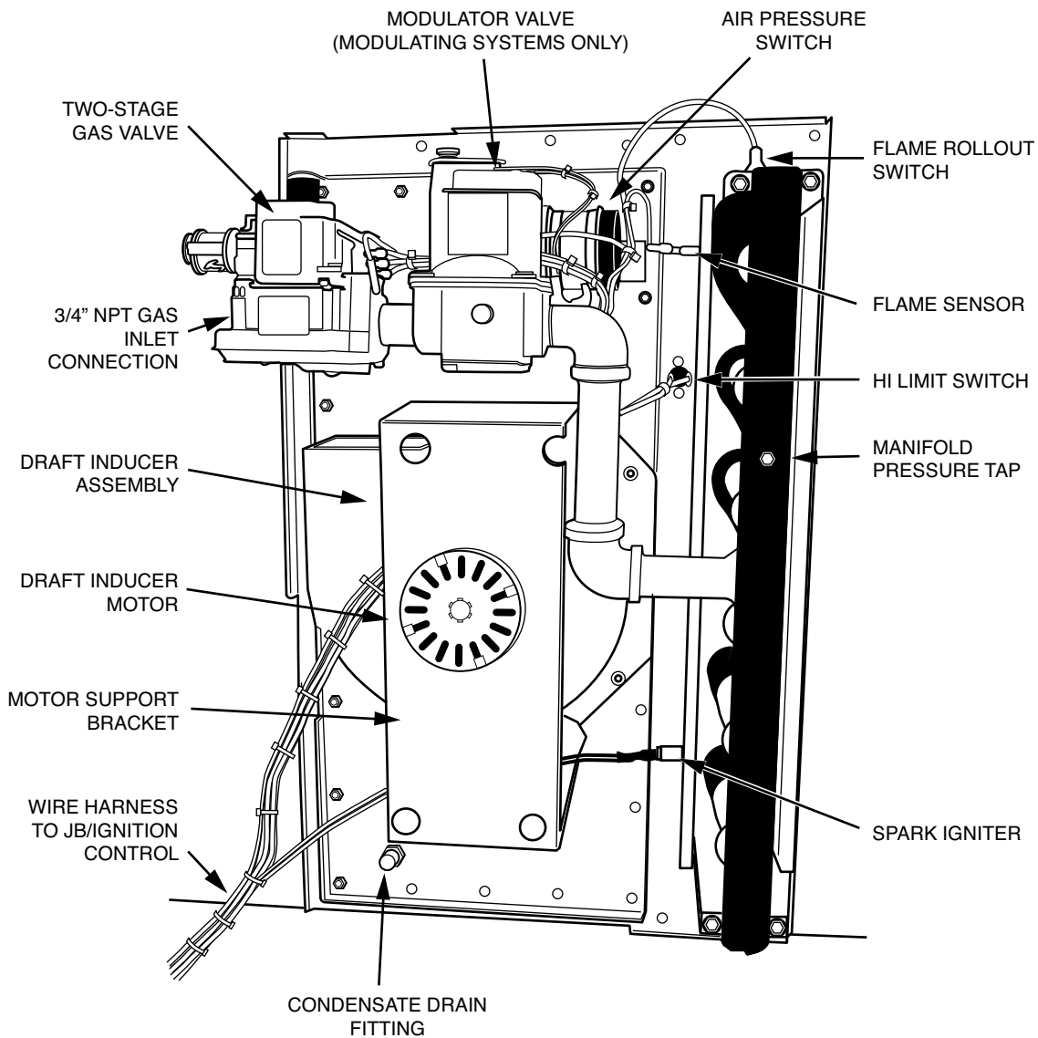
Fig. 144 — Gas-Fired Duct Furnace Components
