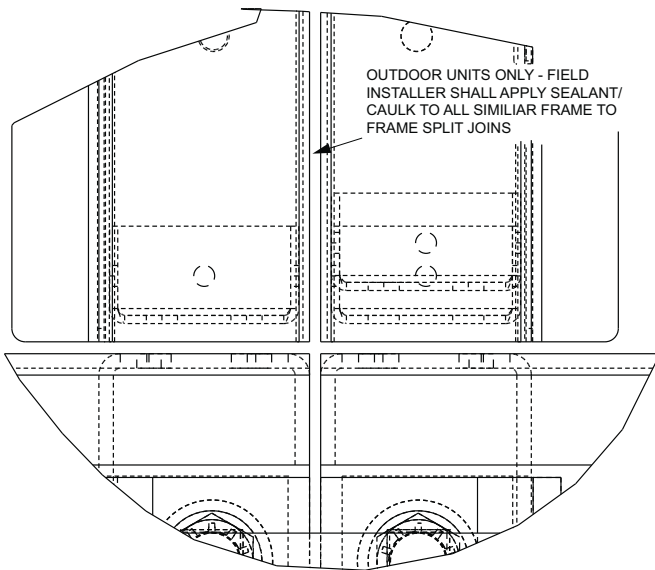
Fig. 168 — Frame to Frame Connections
