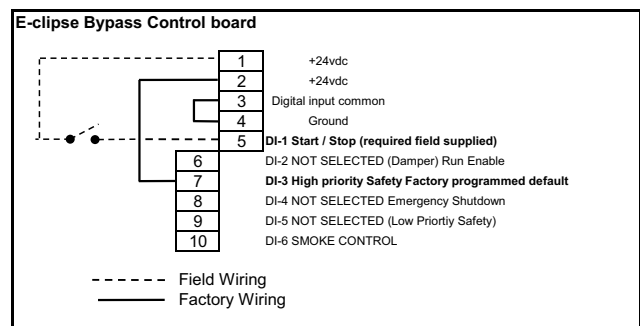
Fig. 134 — E-clipse Bypass Control Board Wiring
