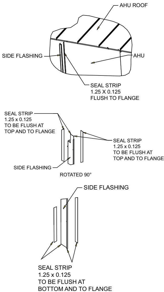
Fig. 62 — Installing Seal Strip
