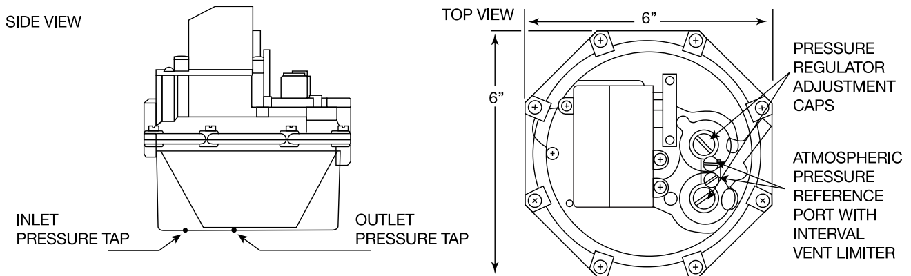
Fig. 152 — Honeywell V8944 Gas Valve
