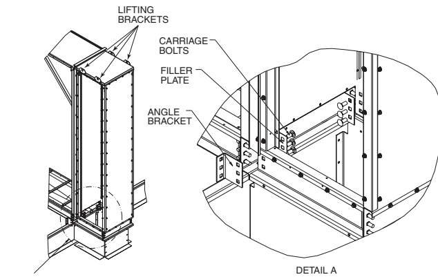
Fig. 70 — Positioning CCH
